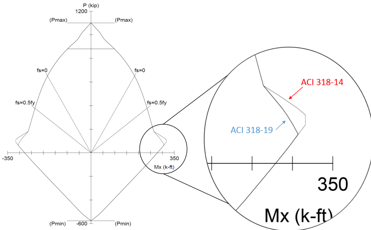
Figure 11 – Design (Factored) Interaction Diagrams using ACI 318-14 and ACI 318-19 ( spColumn )
