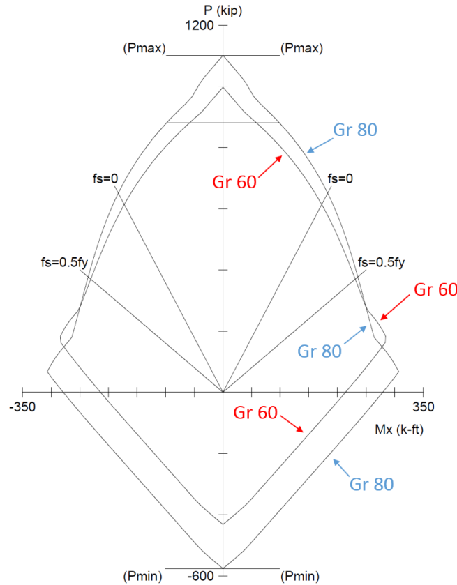
Figure 12 – Design (Factored) Interaction Diagrams using Gr 60 and Gr 80 (spColumn)
