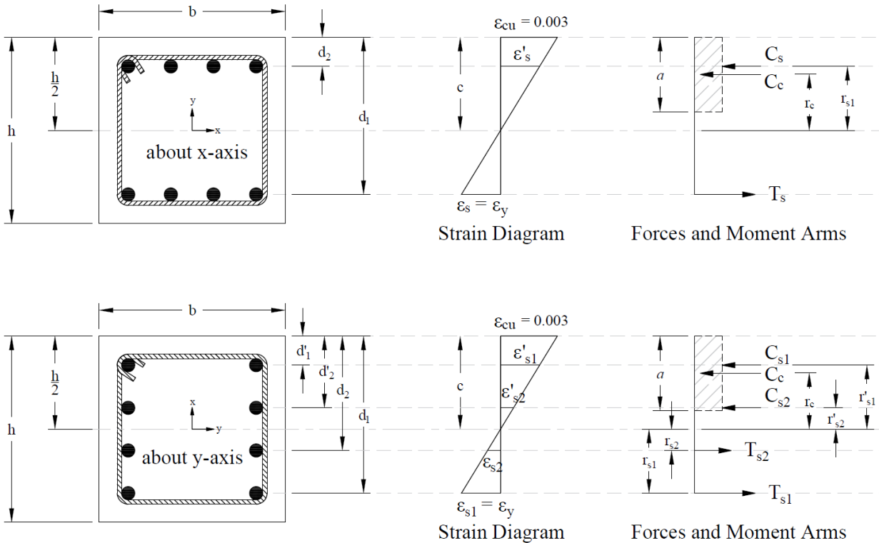
Figure 13 – Strains, Forces, and Moment Arms ( f_s = -f_y Moments About x- and y-axis)
