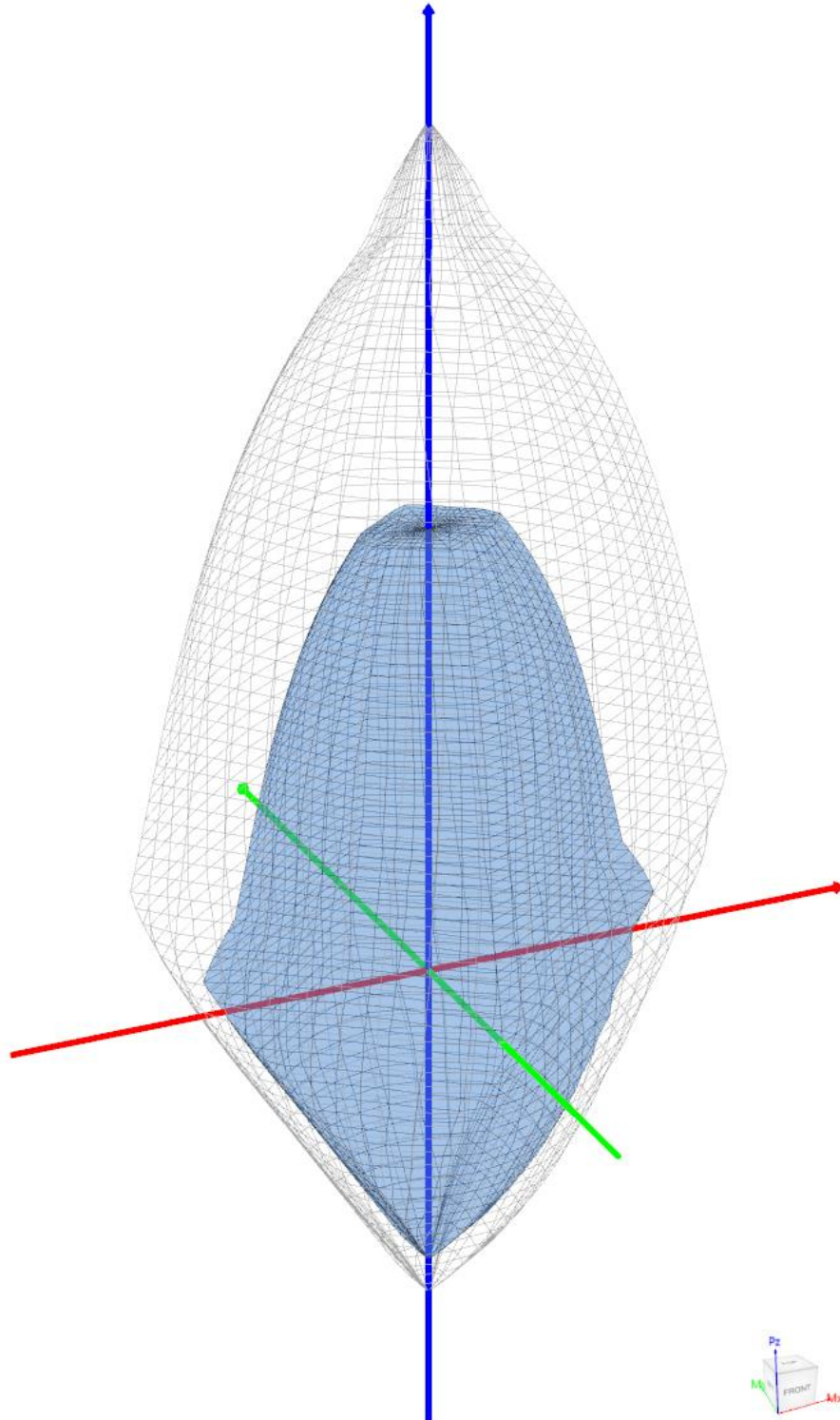
Figure 15 – Nominal & Design Interaction Diagram in Two Directions (Biaxial) (spColumn)
