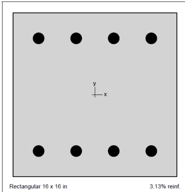
Figure 1: Column section
