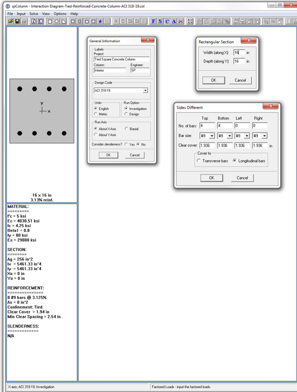
Figure 8 – Generating spColumn Model
