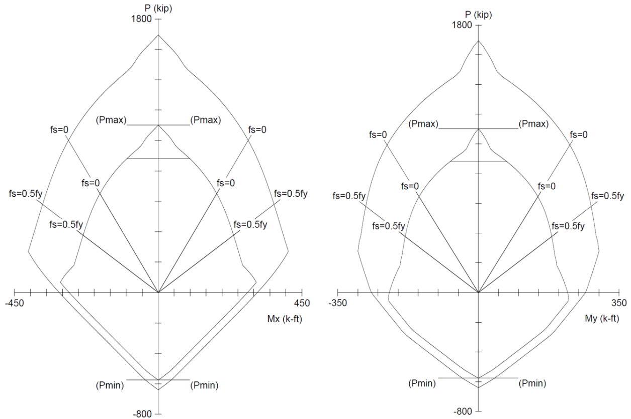
Interaction Diagram About the X-Axis
