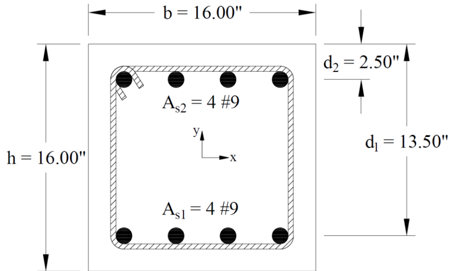
Figure 1 – Reinforced Concrete Column Cross-Section
